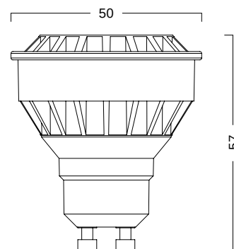
Dimensions (MM)
